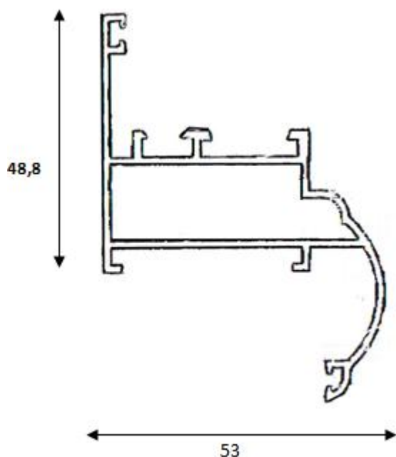
DE1010 | 0,880 Kg/m
